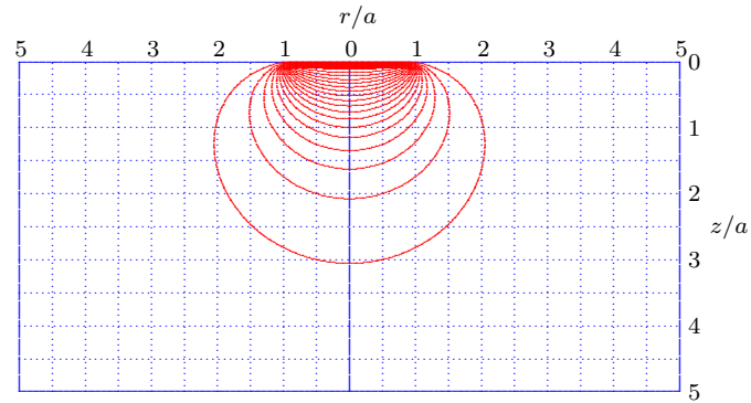
Figure 8.6: ASP : Pore pressure (Analytic), ct/a^2 = 0.0001 .
