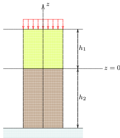
Figure 2.14: Soil consisting of two layers.
