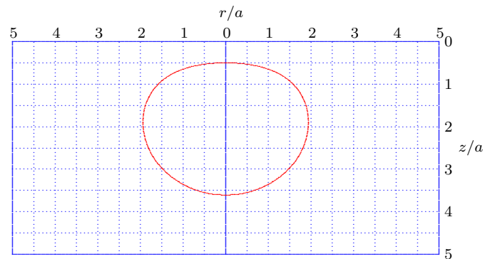
Figure 8.8: ASP : Pore pressure (Analytic), ct/a^2 = 1 .
