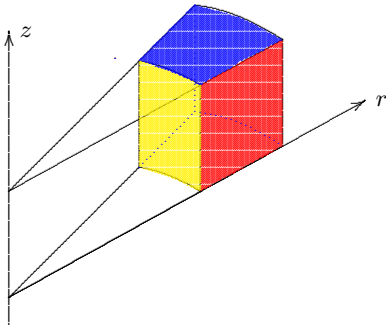
Figure 8.1: Axially symmetric element.
