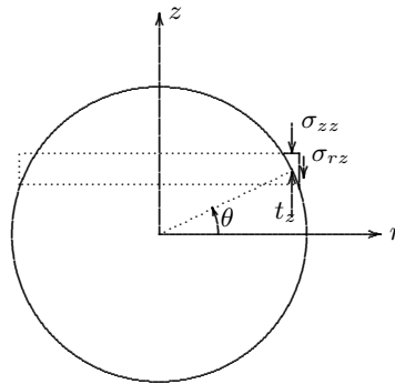
Figure 3.15: Kelvin's problem
