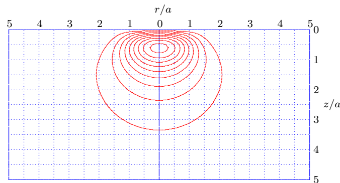
Figure 8.17: ASP : Pore pressure (Talbot), ct/a^2 = 0.1 .
