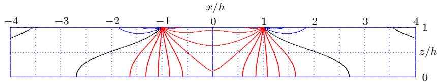
Figure 7.17: PSPL : Isotropic total stress, ct/h^2 = 0.1 .
