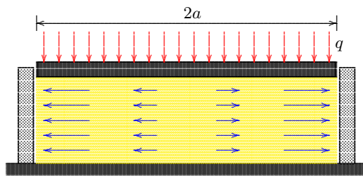
Figure 3.1: Mandel's problem.
