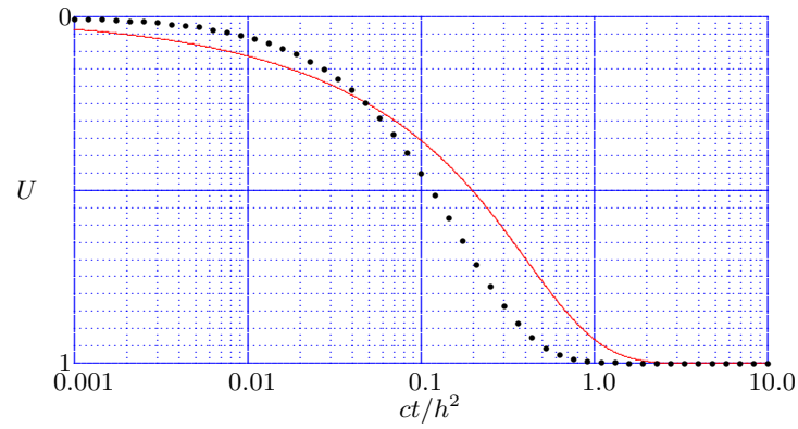
Figure 3.29: Terzaghi's problem : Degree of Consolidation.
