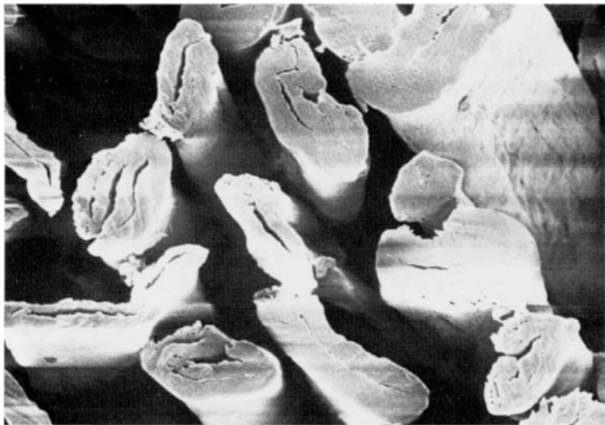
3.1 Cross-section of cotton fibres \times 1500 .
