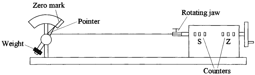
4.9 A tension twist tester.
